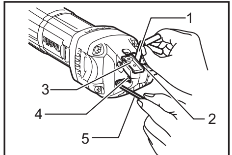
► 1. Thickness gauge 2. Center blade 3. Side blade 4. Hex socket head bolt 5. Hex wrench
